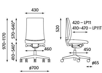
NAVIGO UPH LP11 RTS TS25 (ST44) ESH Weight | Gewicht: 14.55 kg (14.80 kg) NAVIGO MESH/MESH PLUS Weight | Gewicht: 14.05 kg (14.30 kg)
