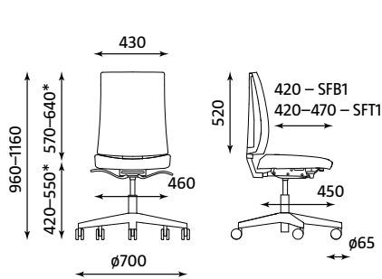
NAVIGO UPH SFB1 RTS TS25 (ST44) ESH Weight | Gewicht: 14.80 kg (15.05 kg) NAVIGO MESH/MESH PLUS Weight | Gewicht: 14.30 kg (14.55 kg)
