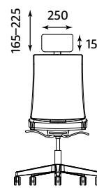
NAVIGO UPH HRUA LP11 RTS TS25 (ST44) ESH Weight | Gewicht: 15.15 kg (15.40 kg) NAVIGO MESH/MESH PLUS Weight | Gewicht: 14.65 kg (14.90 kg)
